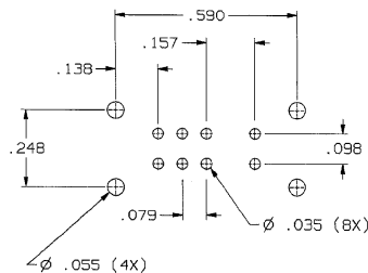
P.C.B. HOLE LAYOUT TOLERANCE FOR P.C.B. HOLE LAYOUT ±.002
