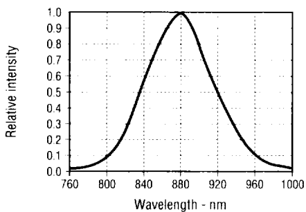
Fig. 5 Spectral Bandwidth
