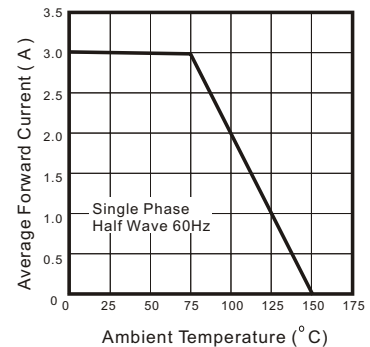
Fig. 6 - Current Derating Curve
