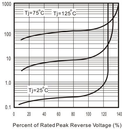
Fig. 1 - Reverse Characteristics
