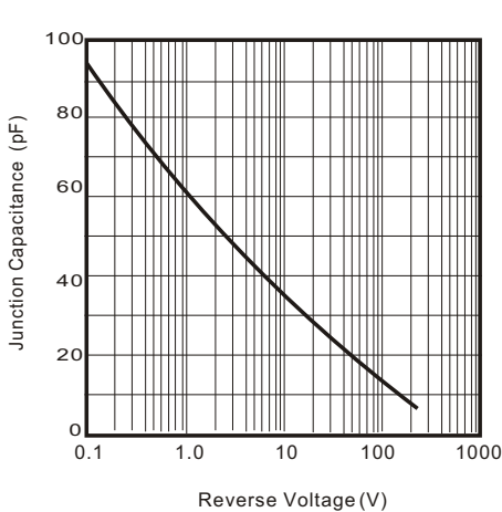
Fig. 3 - Junction Capacitance
