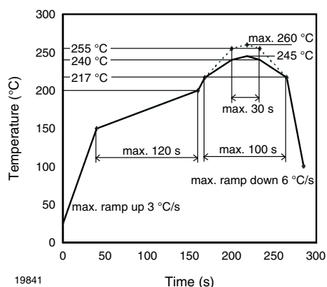
Fig. 27 - Lead (Pb)-free Reflow Solder Profile According to J-STD-020 for SMD Devices
