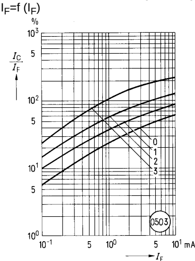
Figure 5. Current transfer ratio versus diode current ( T_A=25\text{ }^\circ\text{C} , V_{CE}=5\text{ V} ) I_C/I_F=f(I_F)
