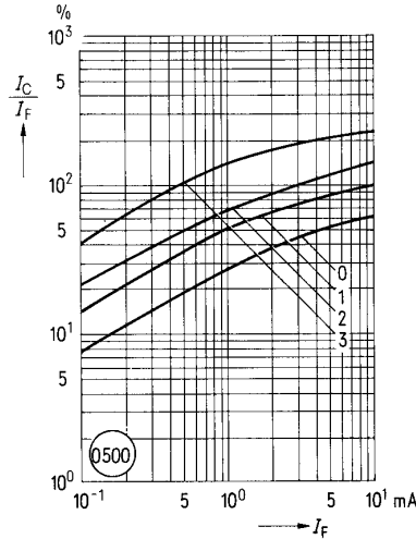
Figure 4. Current transfer ratio versus diode current ( T_A=0\text{ }^\circ\text{C} , V_{CE}=5\text{ V} )
