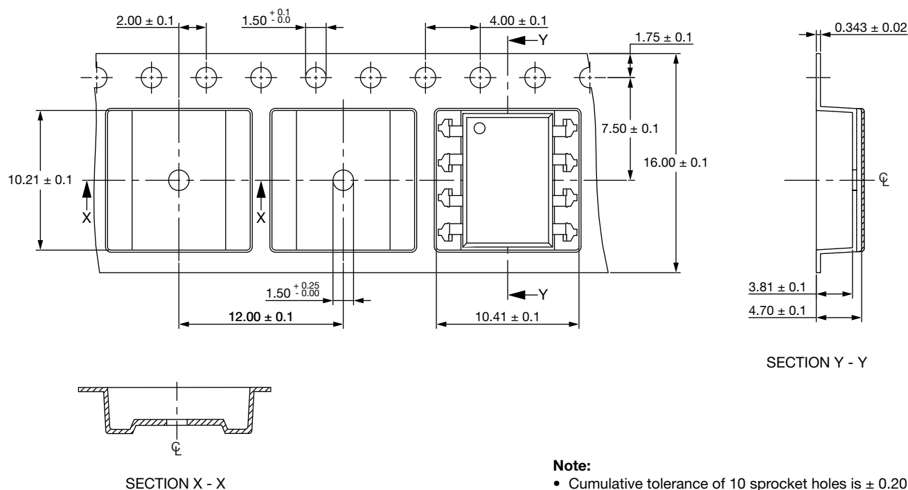
Fig. 12 - Tape and Reel Packing for SMD-8, Option 7 (1000 pieces on reel)
