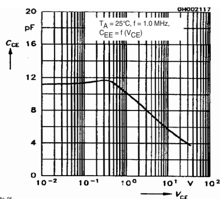
Fig. 7 Transistor Capacitance
