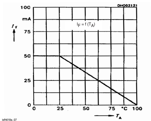
Fig. 9 Permissible Forward Current Diode
