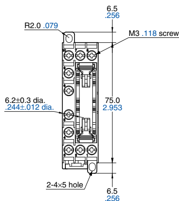
External dimensions
