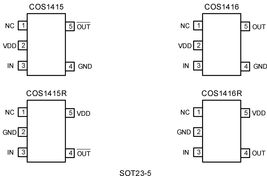
Figure 1. Pin Diagram
