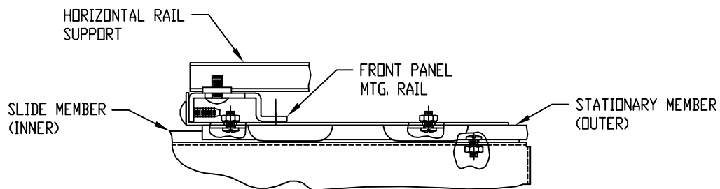
DETAIL "A" DETAIL OF MOUNTING CONFIGURATION
