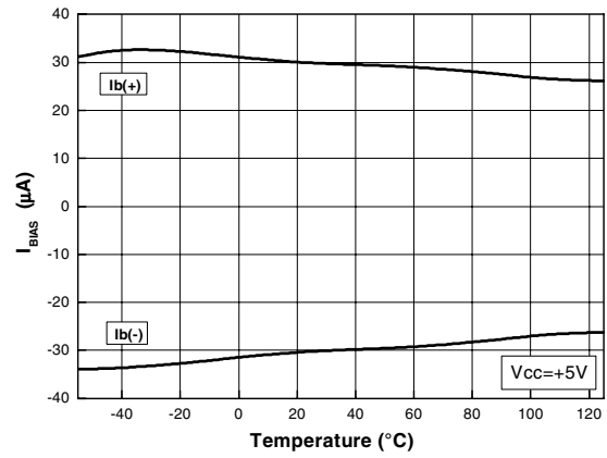
Figure 32. I_{bias} vs. temperature
