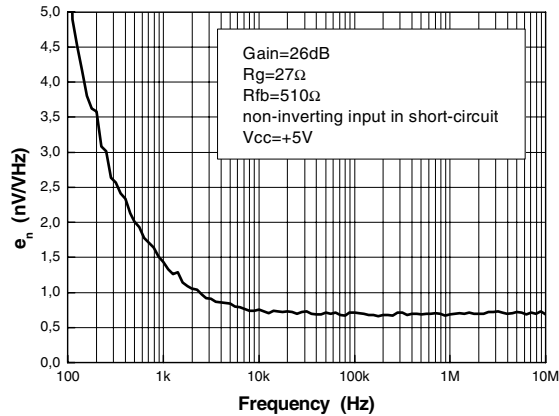
Figure 21. Input voltage noise
