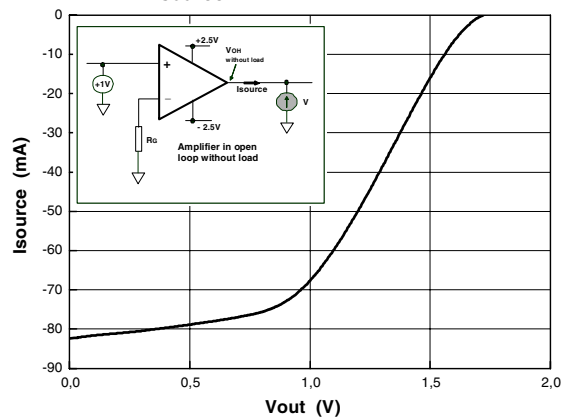
Figure 42. I_{\text{source}}
