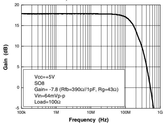
Figure 6. Frequency response G=-7.8, SO8
