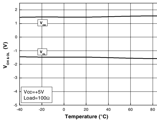
Figure 35. Output rails vs. temperature
