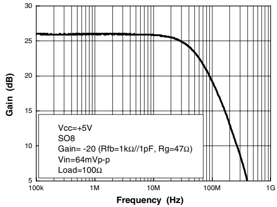
Figure 8. Frequency response G=-19.9, SO8
