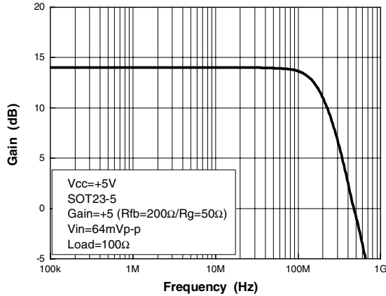
Figure 9. Frequency response G=+5, SOT23-5L
