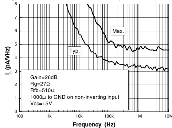
Figure 24. Input current noise (corner lot)
