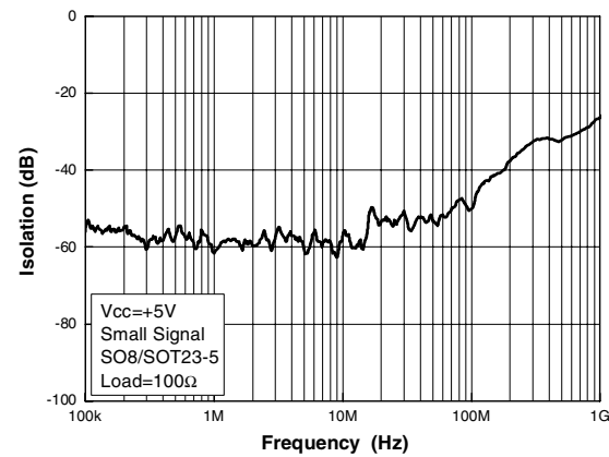
Figure 28. Reverse isolation vs. frequency
