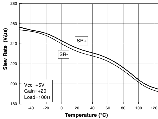
Figure 39. Slew-rate vs. temperature
