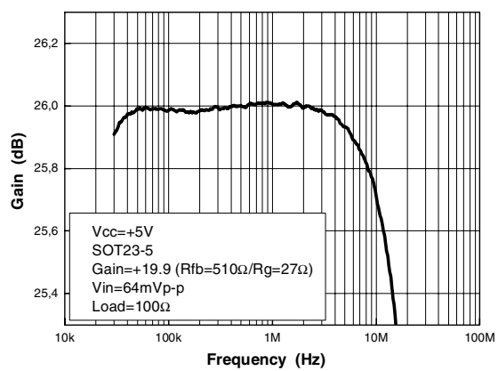
Figure 20. Gain flatness, G=+19.9 , SOT23-5L
