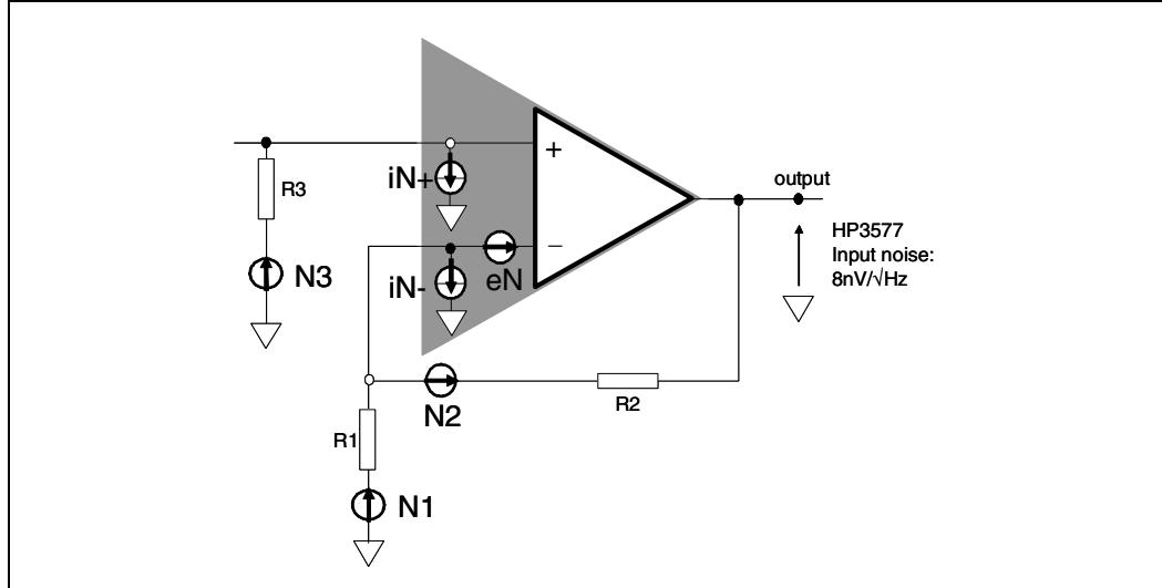
Figure 45. Noise model
