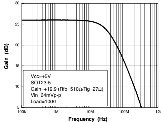
Figure 12. Frequency response G=+19.9, SOT23-5L
