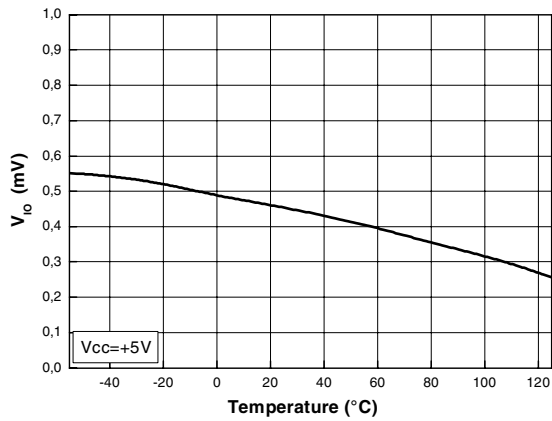
Figure 31. V_{IO} vs. temperature
