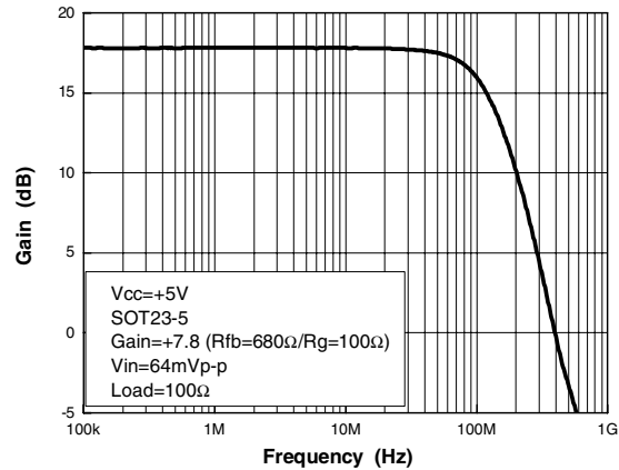
Figure 10. Frequency response G=+7.8, SOT23-5L
