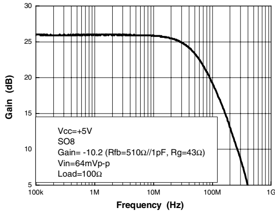
Figure 7. Frequency response G=-10.2, SO8
