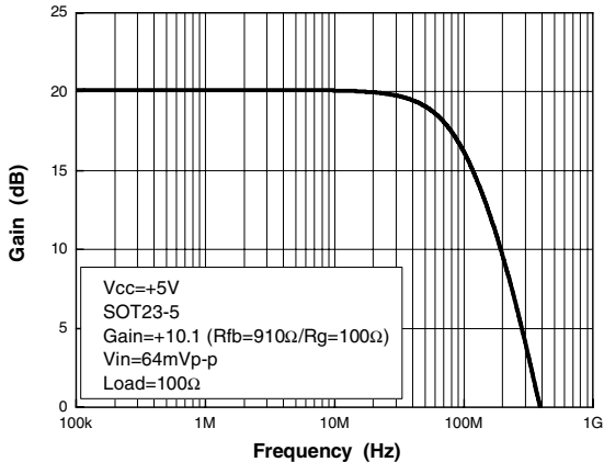
Figure 11. Frequency response G=+10.1, SOT23-5L
