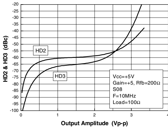
Figure 25. Distortion vs. V_{out} , SO8
