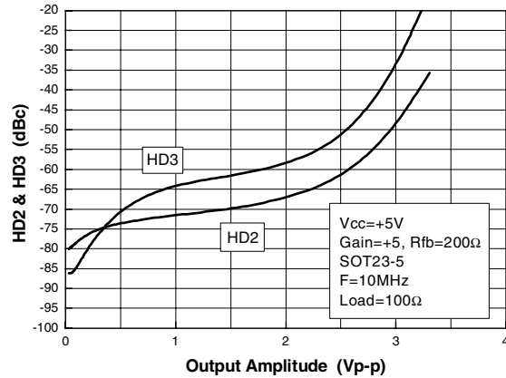
Figure 26. Distortion vs. V_{out} , SOT23-5L
