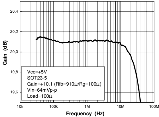
Figure 19. Gain flatness, G=+10.1 , SOT23-5L
