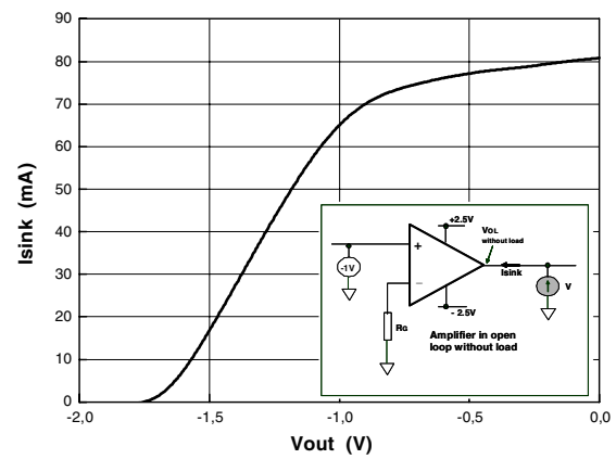
Figure 40. I_{\text{sink}}
