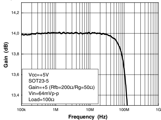
Figure 17. Gain flatness, G=+5 , SOT23-5L
