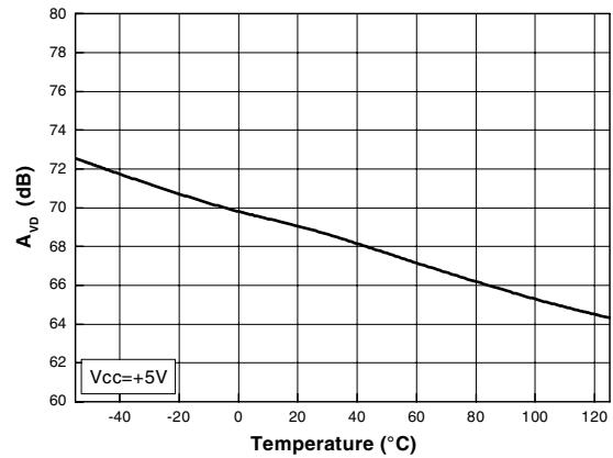
Figure 34. AVD vs. temperature
