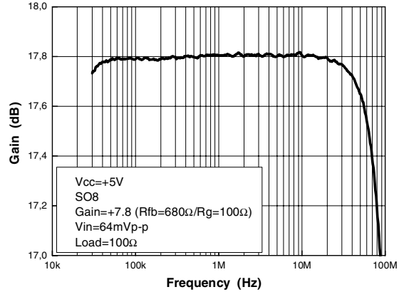
Figure 14. Gain flatness, G=+7.8 , SO8
