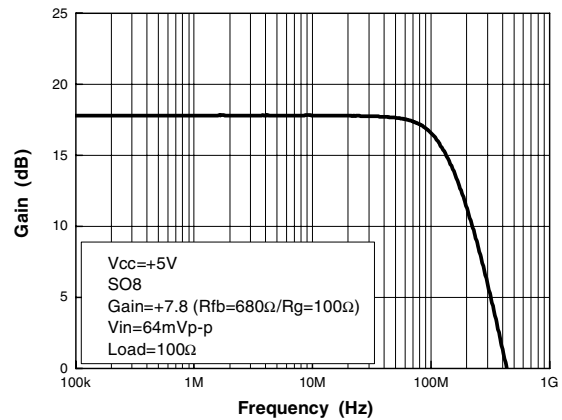
Figure 2. Frequency response G=+7.8, SO8
