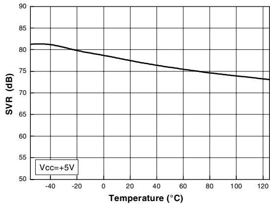
Figure 41. SVR vs. temperature
