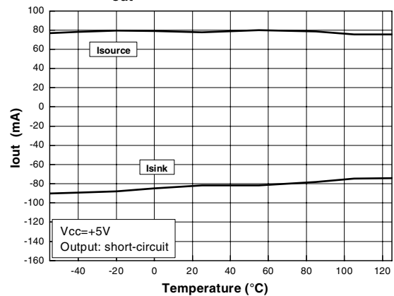
Figure 36. I_{out} vs. temperature
