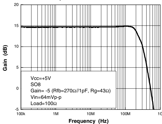
Figure 5. Frequency response G=-5, SO8
