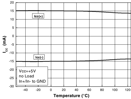
Figure 33. Supply current vs. temperature
