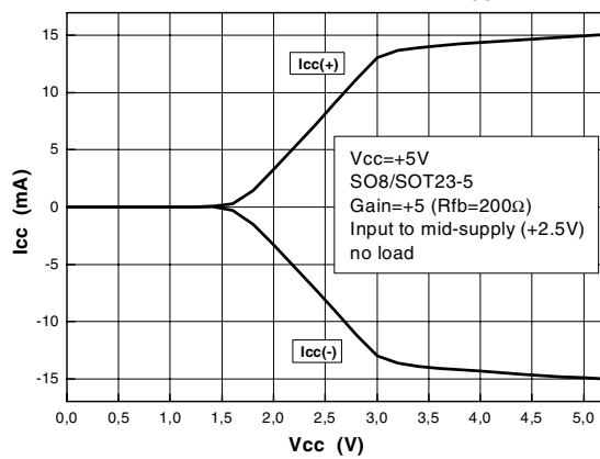
Figure 29. Quiescent current vs. V_{cc}
