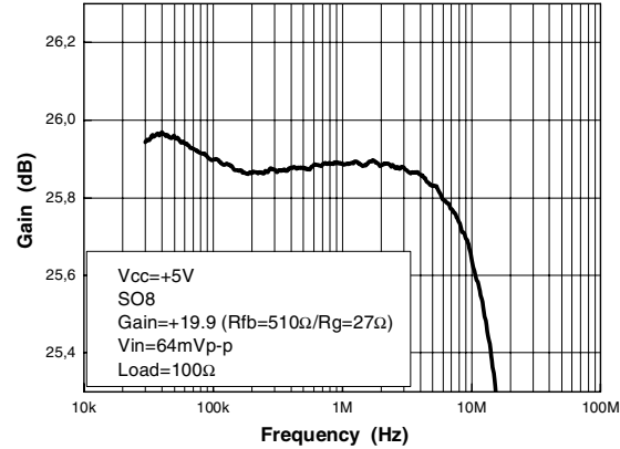
Figure 16. Gain flatness, G=+19.9 , SO8
