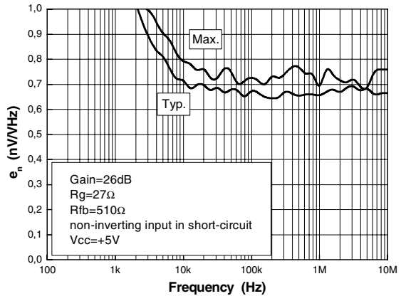
Figure 22. Input voltage noise (corner lot)
