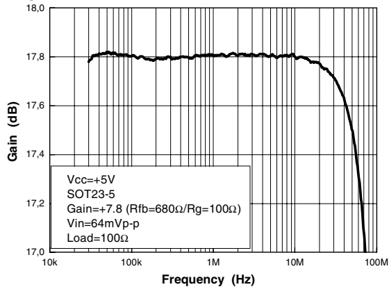
Figure 18. Gain flatness, G=+7.8 , SOT23-5L
