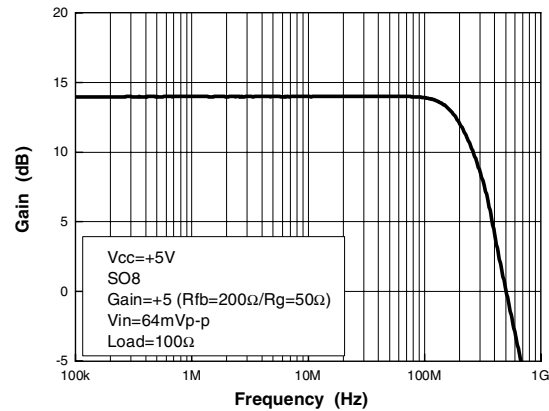
Figure 1. Frequency response G=+5, SO8
