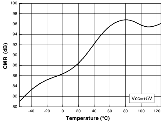
Figure 37. CMR vs. temperature
