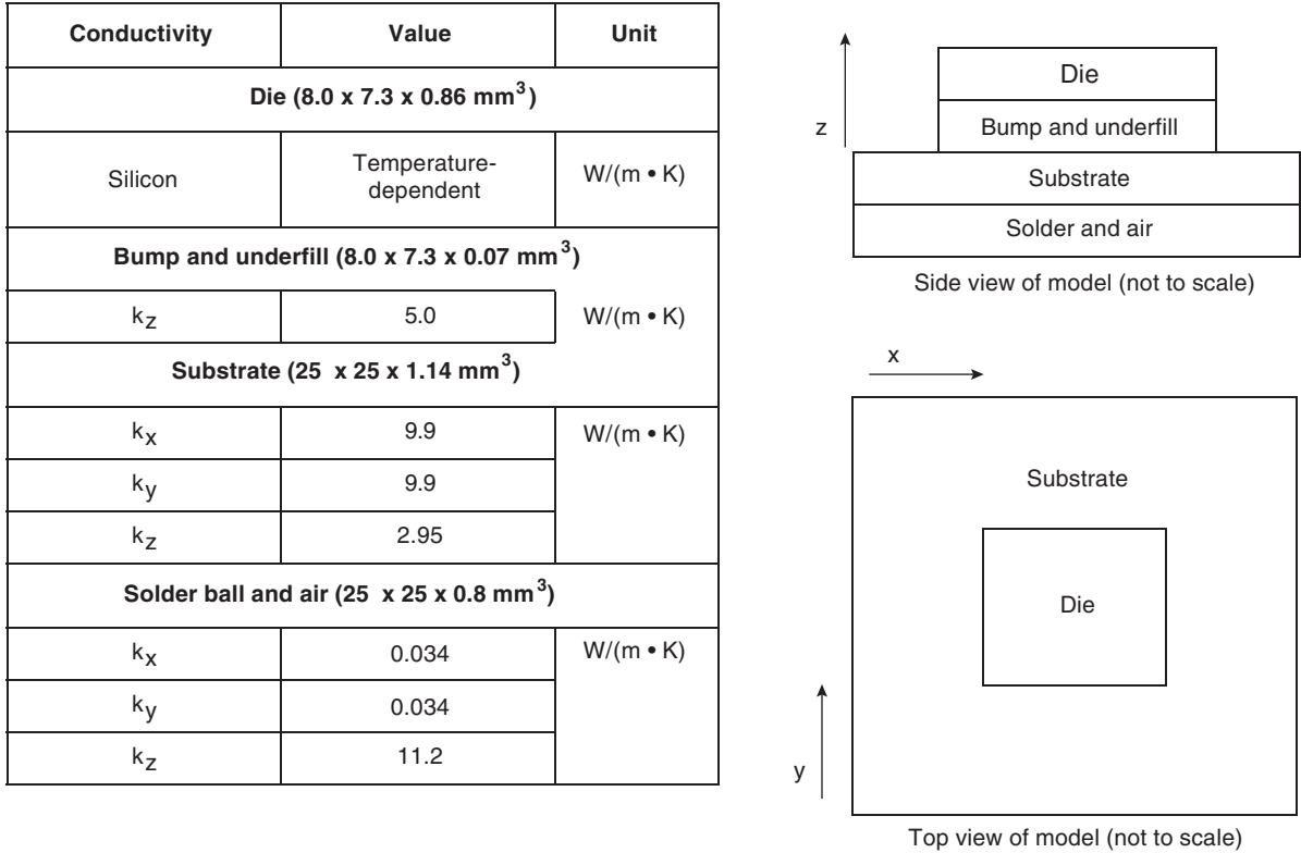
Figure 9-11. Recommended Thermal Model of PC7448
