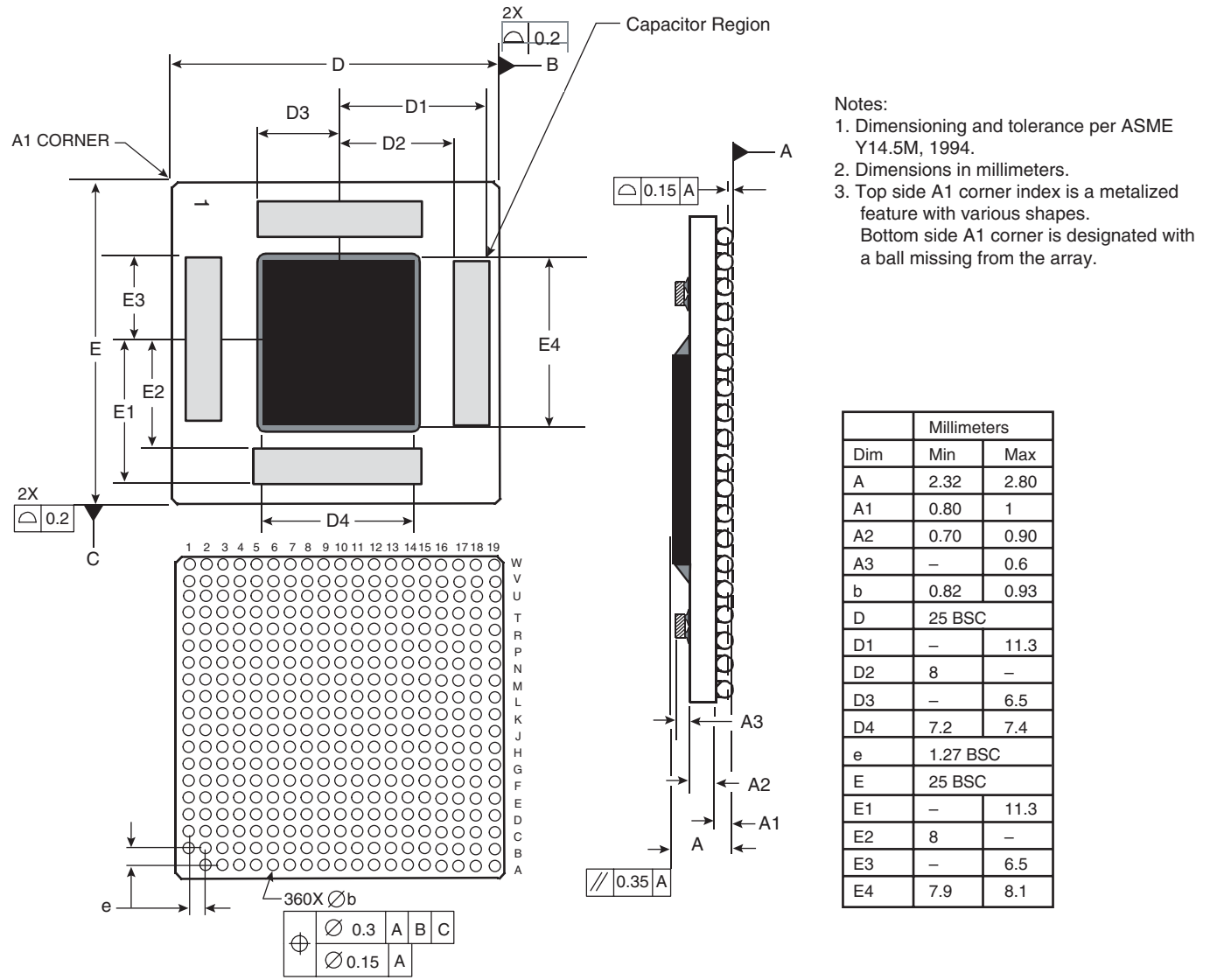
Figure 8-1. Mechanical Dimensions and Bottom Surface Nomenclature for the PC7448, 360 HiTCE BGA Package
