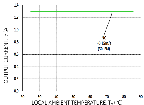
Figure 15. Output Current Derating for the Open Frame SHHD001A3B in the Transverse Orientation; Airflow Direction from Vin(-) to Vin(+); Vin = 48V.
