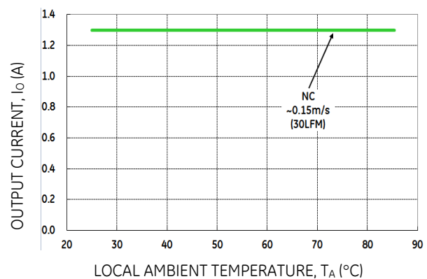
Figure 14. Output Current Derating for the Open Frame SHHD001A3B in the Transverse Orientation; Airflow Direction from Vin(-) to Vin(+); Vin = 24V.
