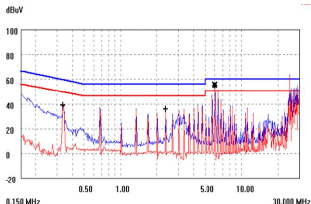
Figure 18. EMC signature using above filter, SHHDA.
