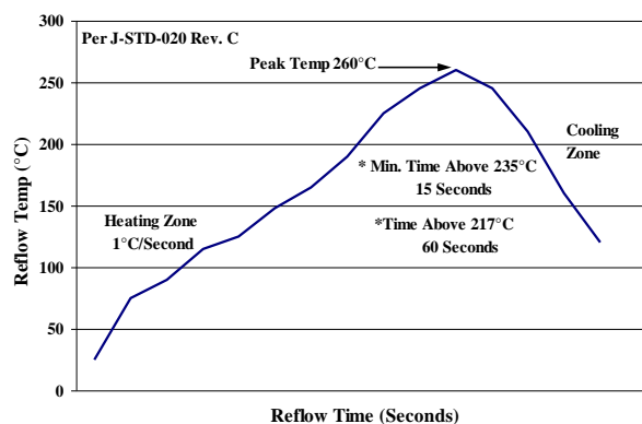
Figure 22. Recommended linear reflow profile using Sn/Ag/Cu solder.
