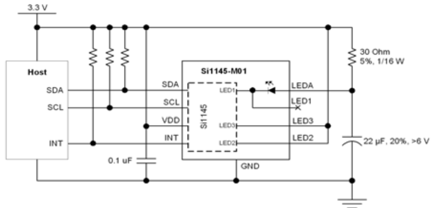
Figure 2. Si1145-M01 Module Basic Application Schematic for 1 LED
