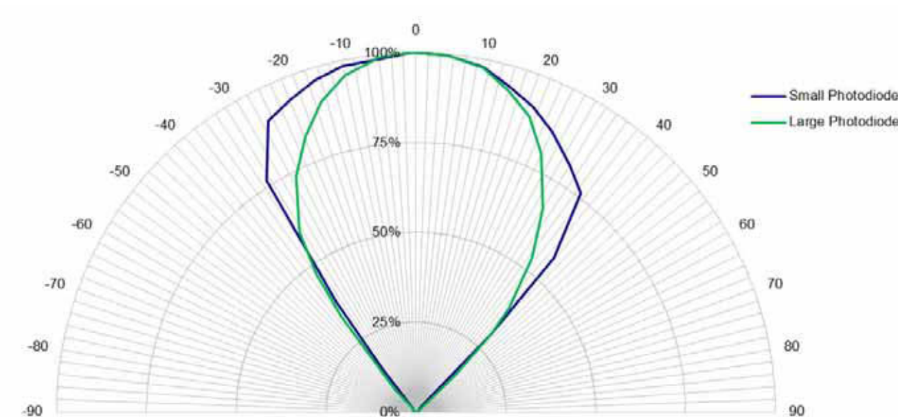
Figure 11. Transverse Photodiode View Angle
