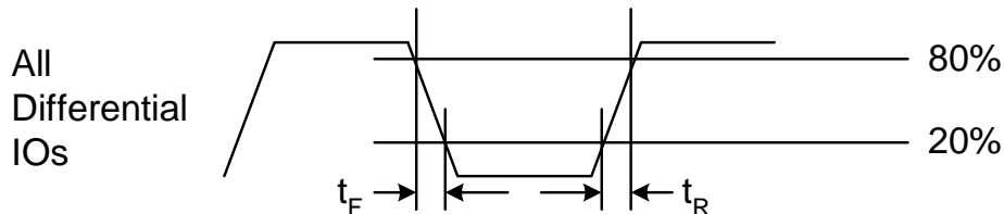
Figure 3. I/O Rise/Fall Times
