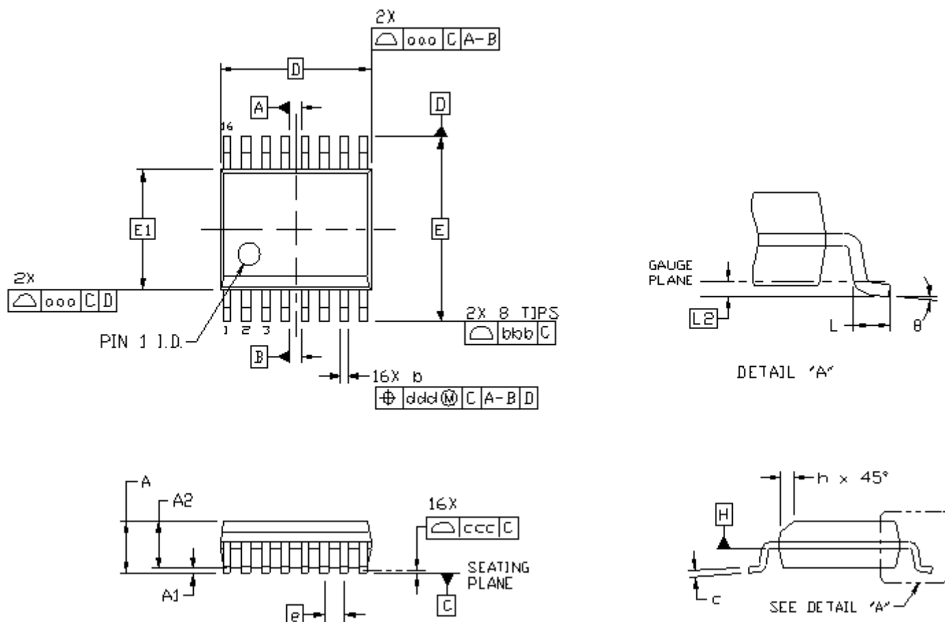
Figure 10.1. 16-Pin QSOP
