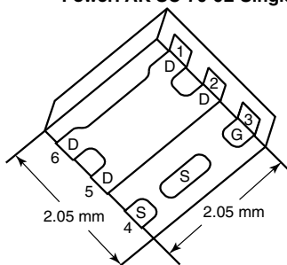
PowerPAK SC-70-6L-Single
