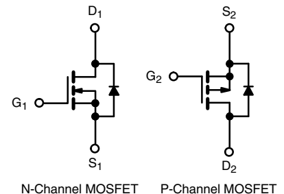
N-Channel MOSFET
