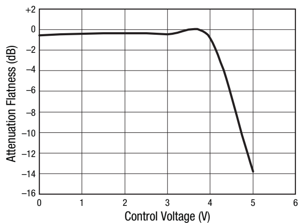
Figure 5. Attenuation Flatness vs Control Voltage ( f = 2.1 to 3.1\text{ GHz} )
