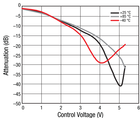
Figure 4. Attenuation vs Control Voltage Over Temperature ( f = 2.6\text{ GHz} )
