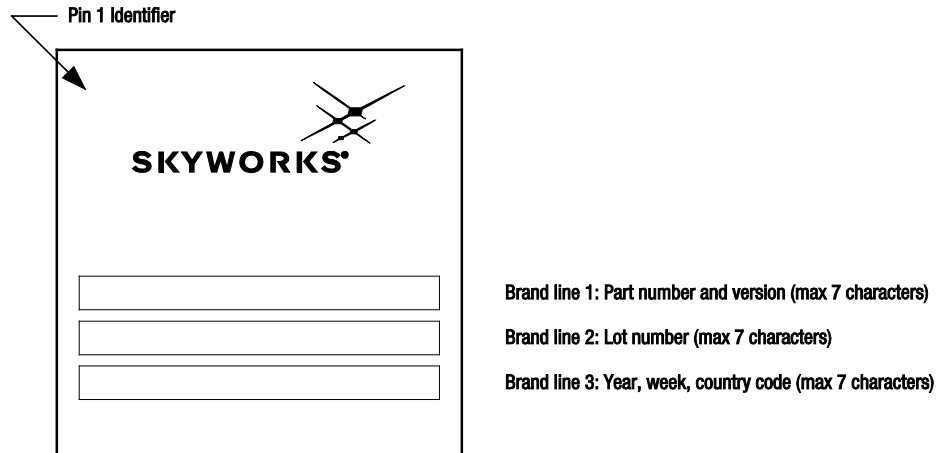
Figure 8. Typical Case Markings (Top View)
