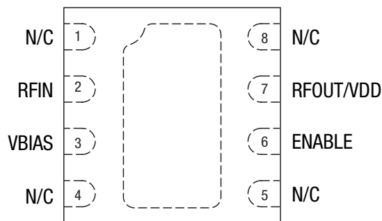
Figure 2. SKY67153-396LF Pinout – 8-Pin DFN (Top View)
