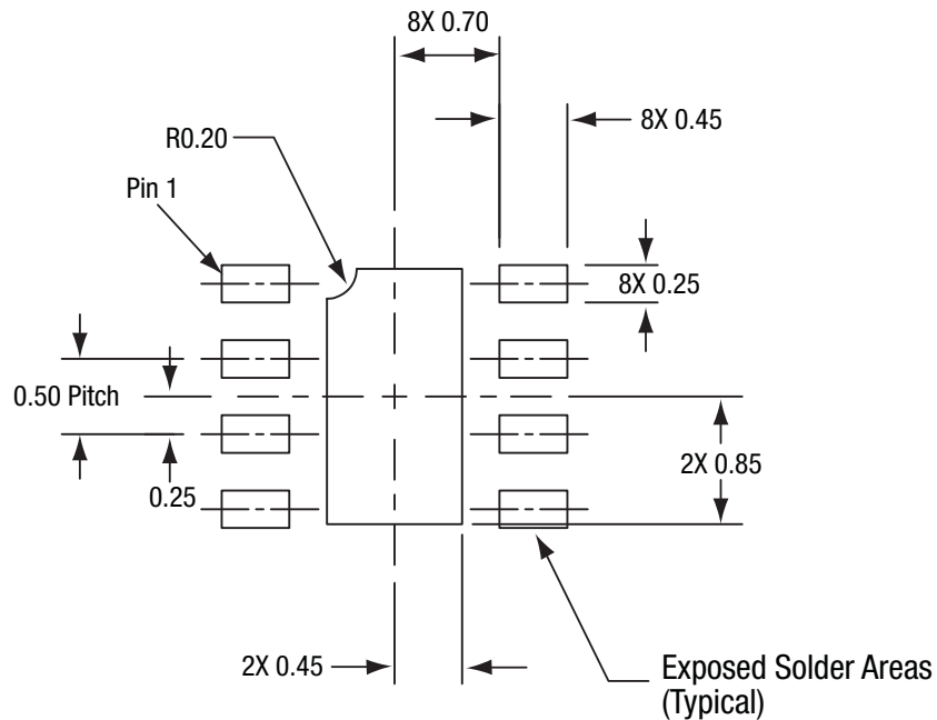
Figure 25. SKY67153-396LF PCB Layout Footprint (Top View)
