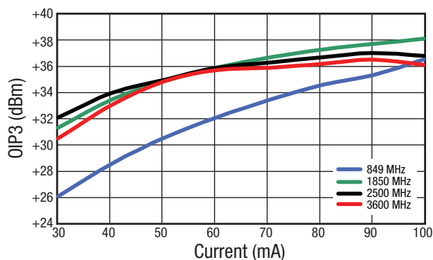
Figure 15. OIP3 vs Quiescent Current Over Frequency Using Band-Specific BOM
