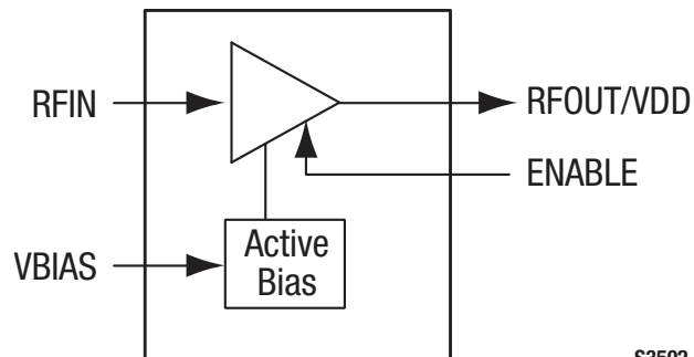
Figure 1. SKY67153-396LF Block Diagram
