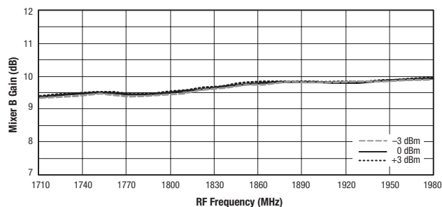
Figure 8. Mixer B Gain vs Frequency and LO Power
