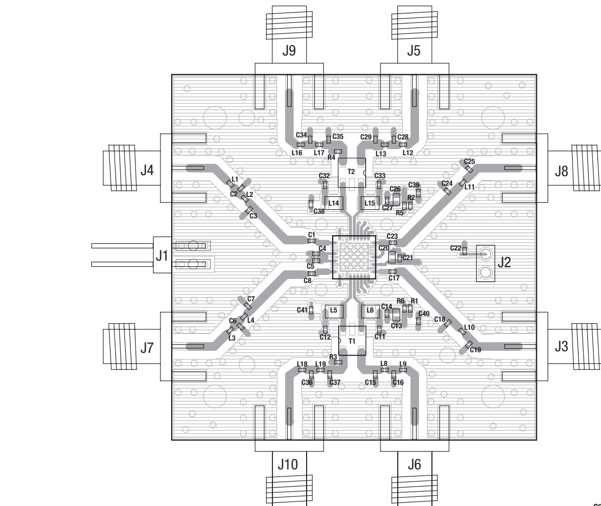
Figure 35. SKY73023-11 Evaluation Board Assembly Diagram
