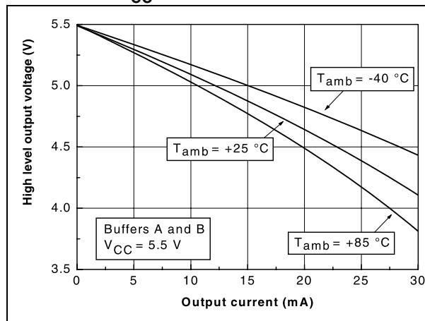
Figure 12. Voltage output high ( V_{OH} ) vs. output current - buffers A and B, V_{CC} = 5\text{ V}
