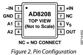
Figure 2. Pin Configuration
