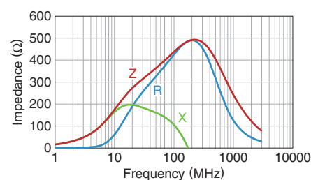
MMZ1608S202ATA00
