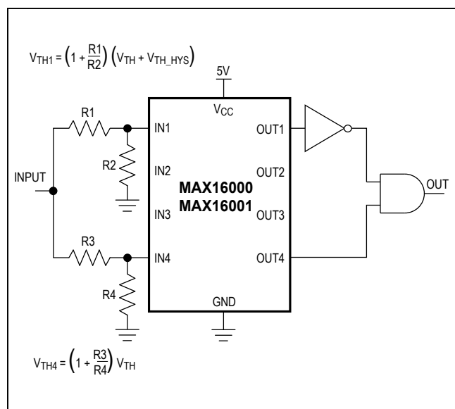
Figure 8. Window Detection
