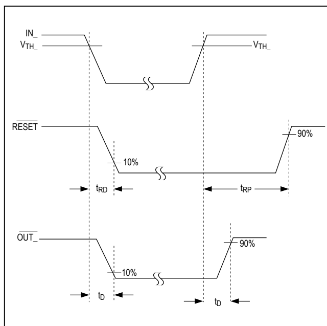
Figure 12. Output Timing Diagram
