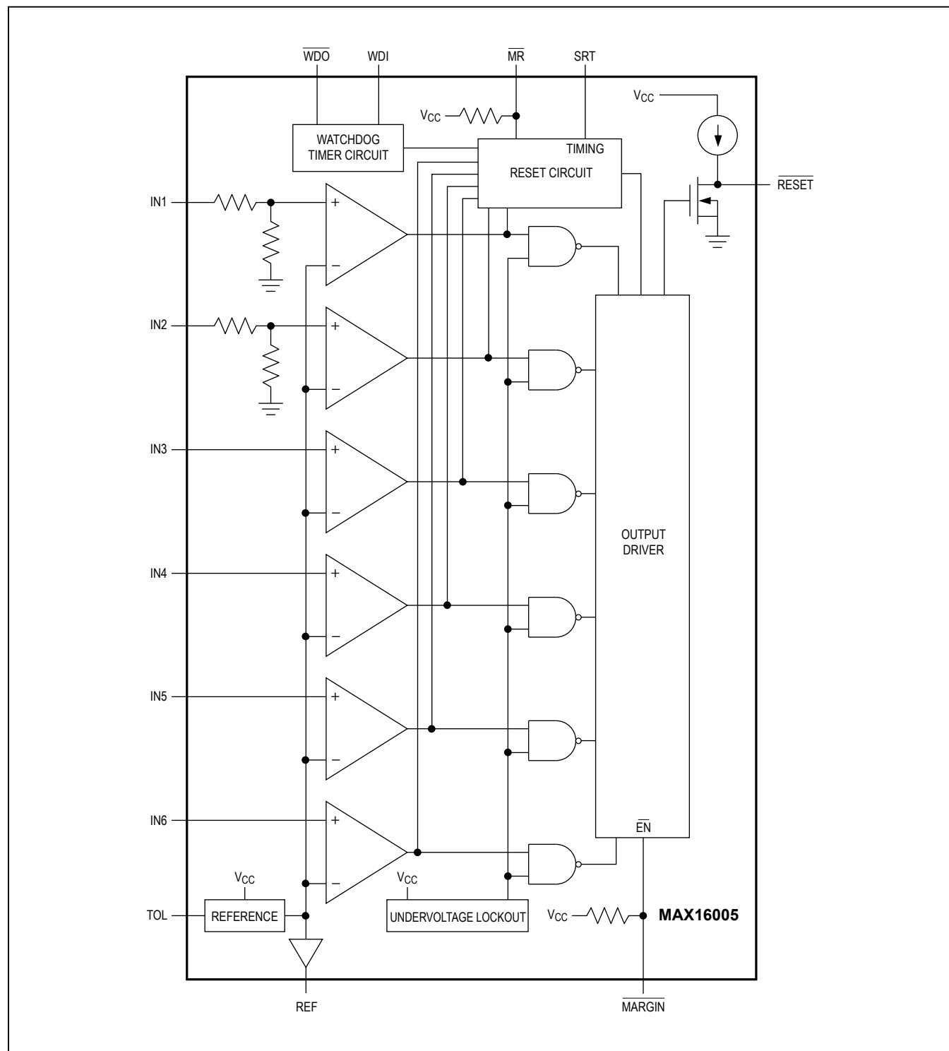
Figure 4. MAX16005C Functional Diagram
