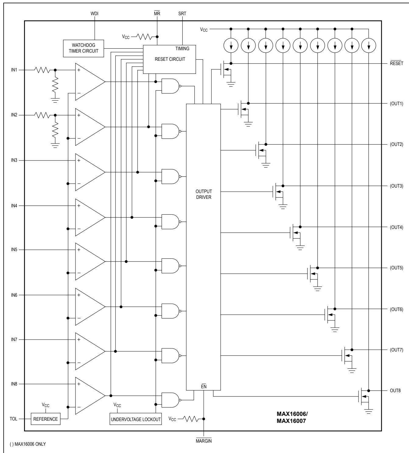
Figure 5. MAX16006C/MAX16007C Functional Diagram
