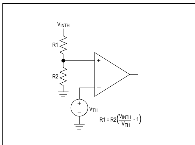
Figure 10. Setting the Adjustable Input
