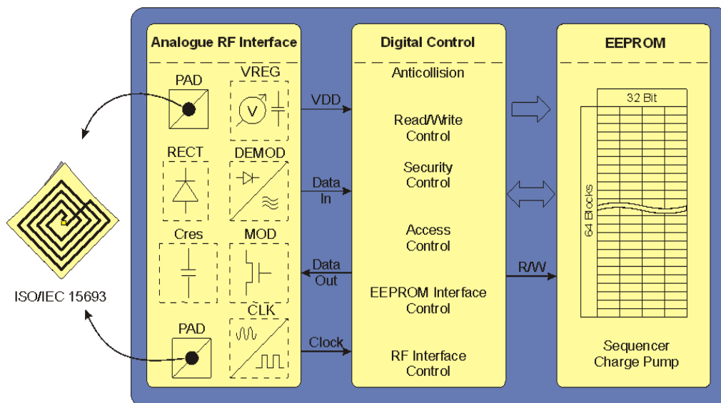
Fig 1. Block diagram of label IC
