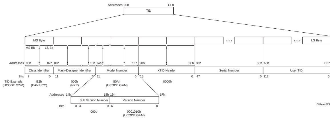
Fig 5. G2iM TID memory structure
