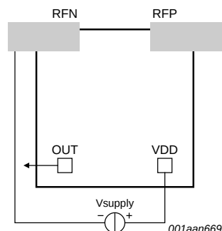
Fig 7. Schematic of external power supply
