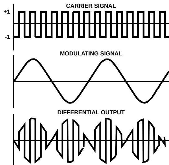
FIGURE 1. TYPICAL MODULATOR SIGNALS
