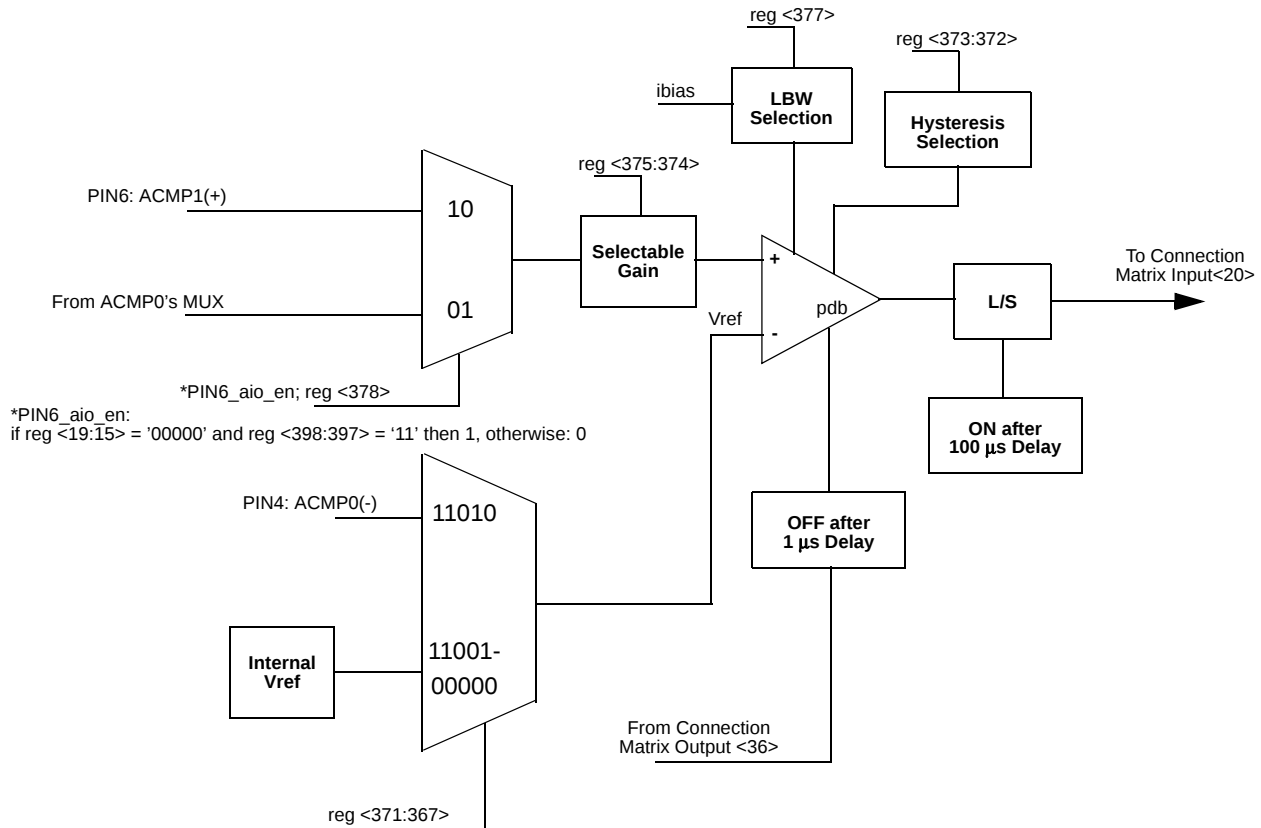
Figure 18. ACMP1 Block Diagram
