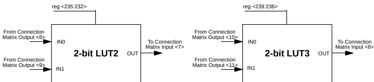
Figure 6. 2-bit LUTs
