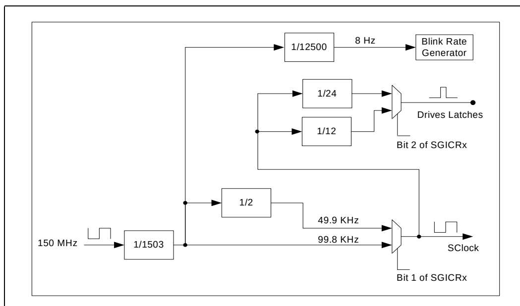
Figure 5-23. Clock Structure
