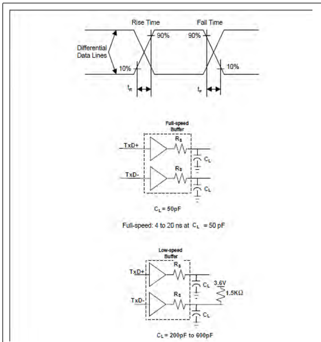
Figure 8-17. USB Rise and Fall Times
