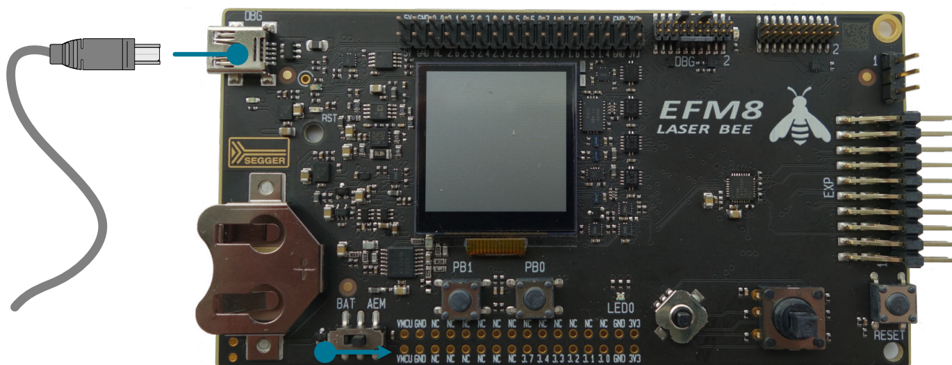
Figure 1.1. Hardware Setup
