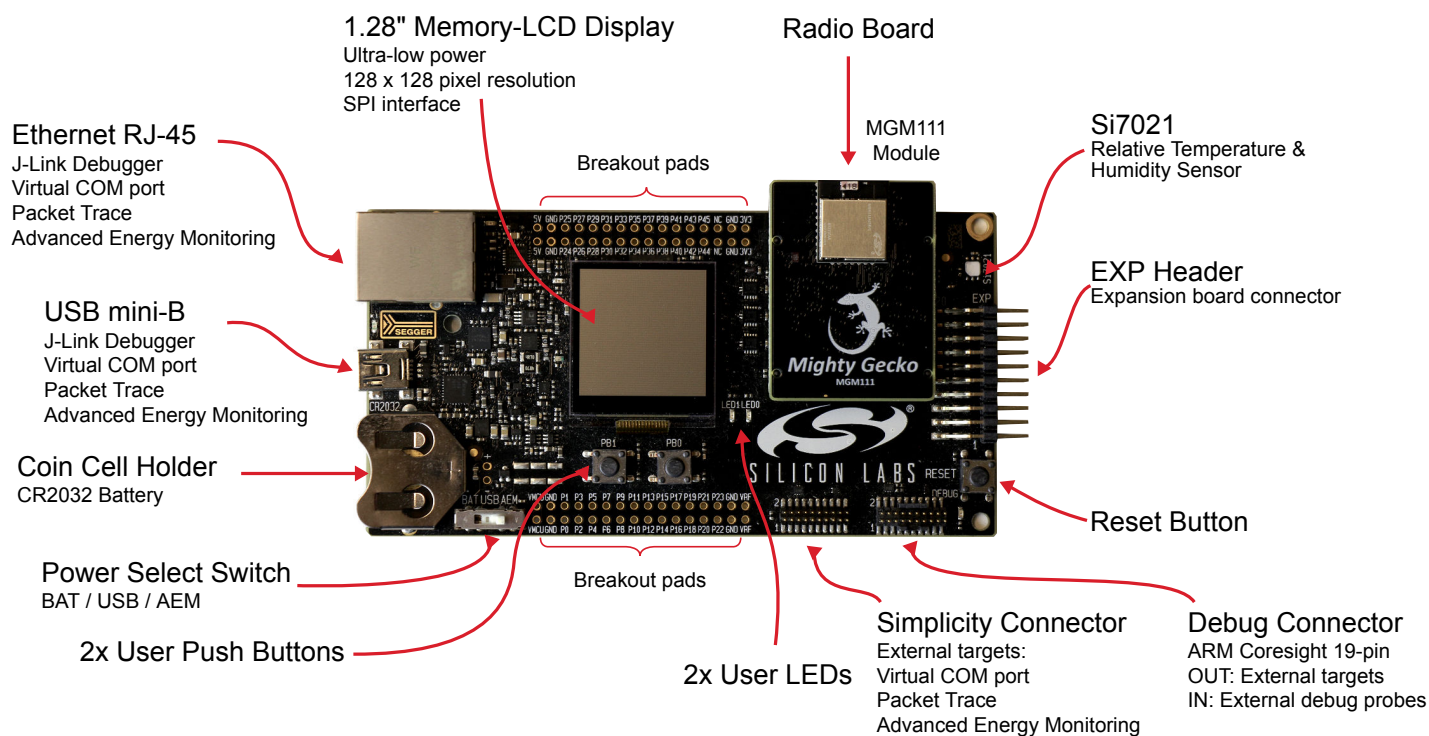
Figure 2.1. SLWRB4300B with Wireless STK Mainboard
