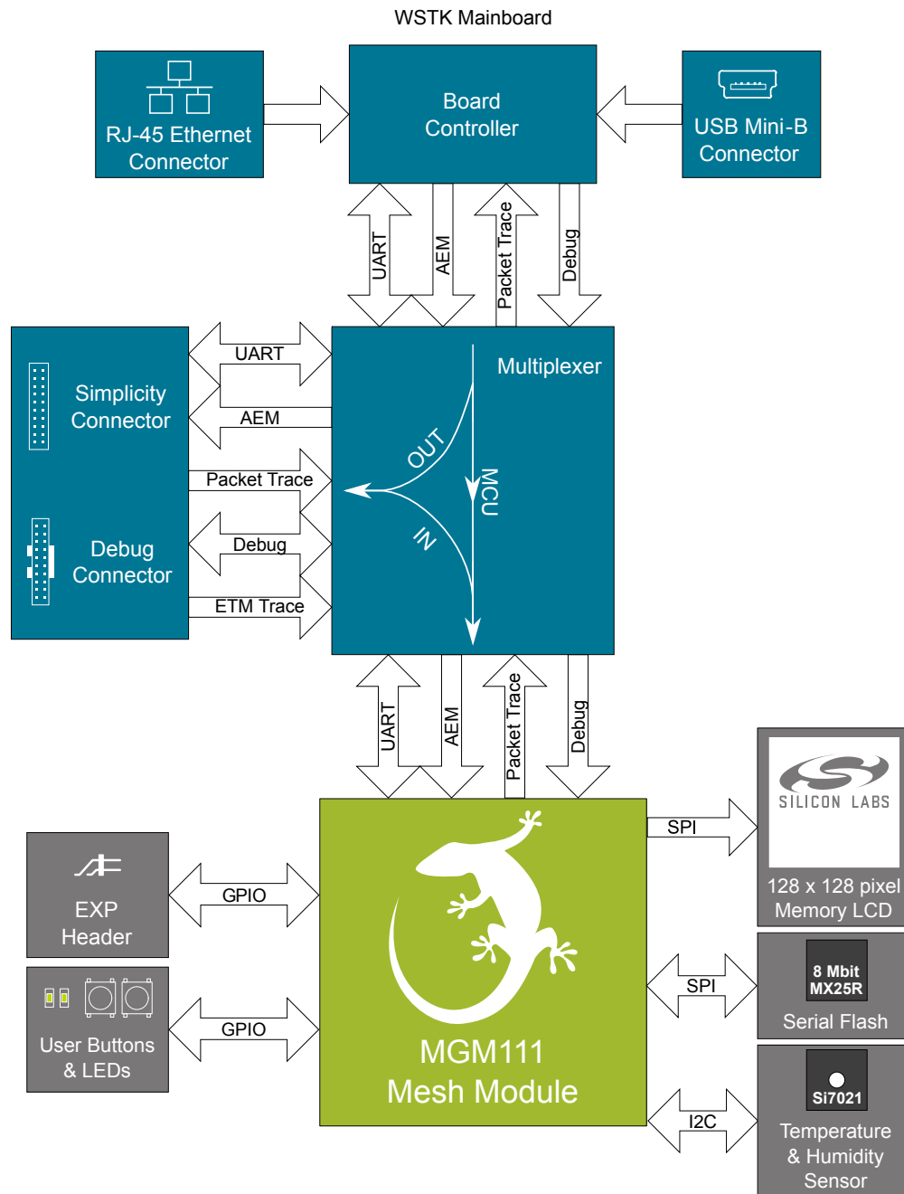
Figure 3.1. Kit Block Diagram
