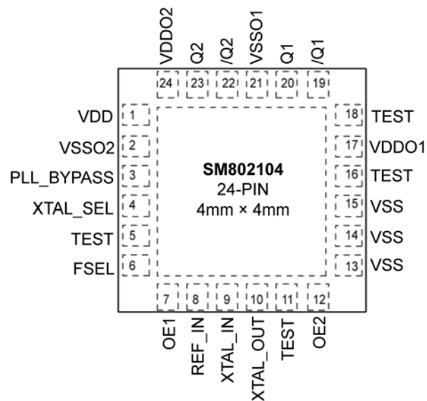
24-Pin QFN (code) (Top View)
