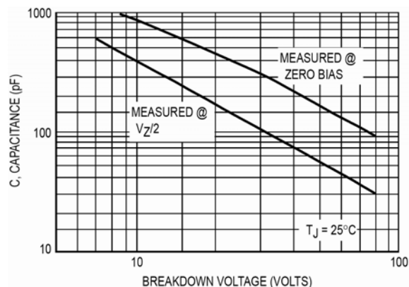
Figure 7. Capacitance curve
