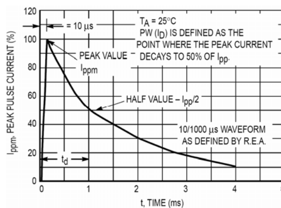
Figure 9. Pulse waveform
