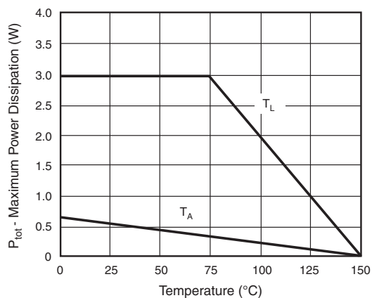
Fig. 1 - Steady State Power Duriating
