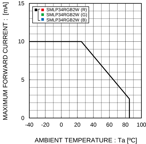
Fig.5 Derating
