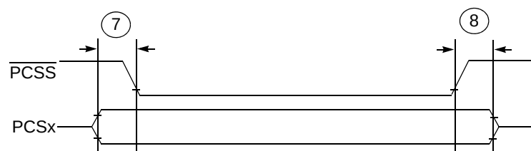
Figure 37. DSPI modified transfer format timing — slave, CPHA = 1
