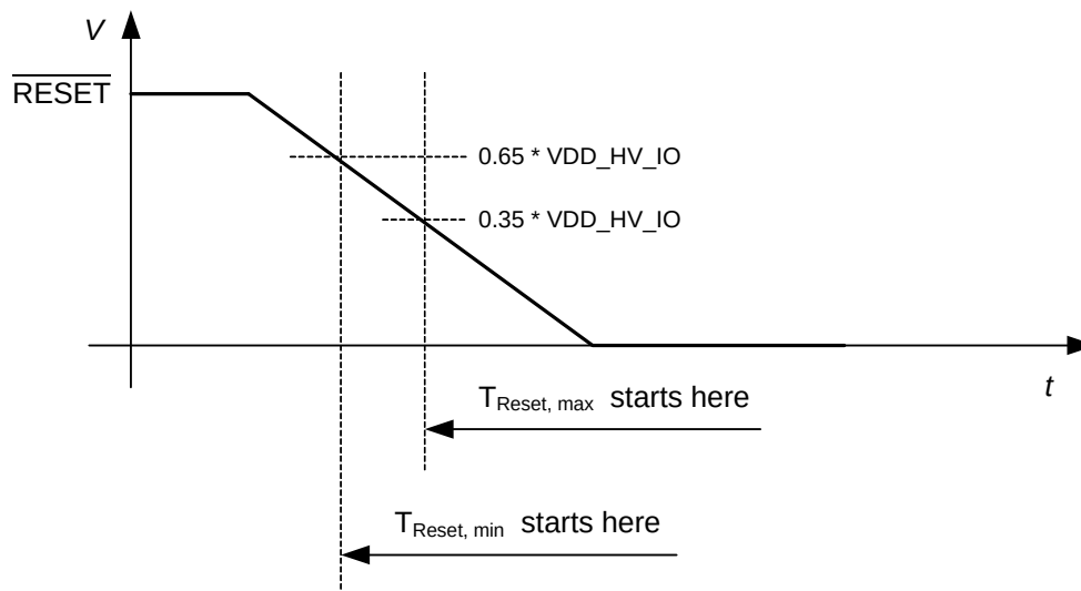
Figure 18. Reset sequence start via RESET assertion
