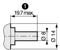
Gearbox shaft 79 206 478
