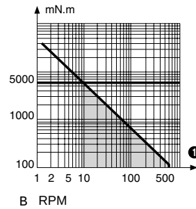
Nominal speed and torque curves 80 815 0
