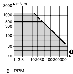
Nominal speed and torque curves
