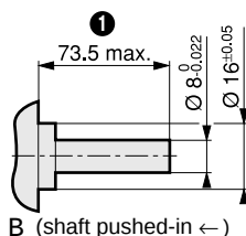
Gearbox shaft 79 290 064
