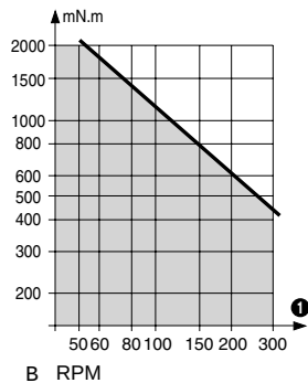
Nominal speed and torque curves 80 803 0
