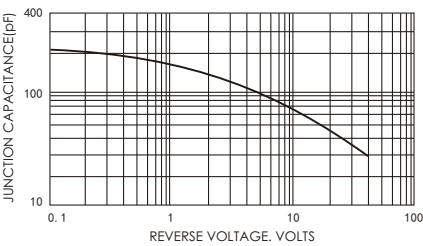
FIG.5-TYPICAL JUNCTION CAPACITANCE
