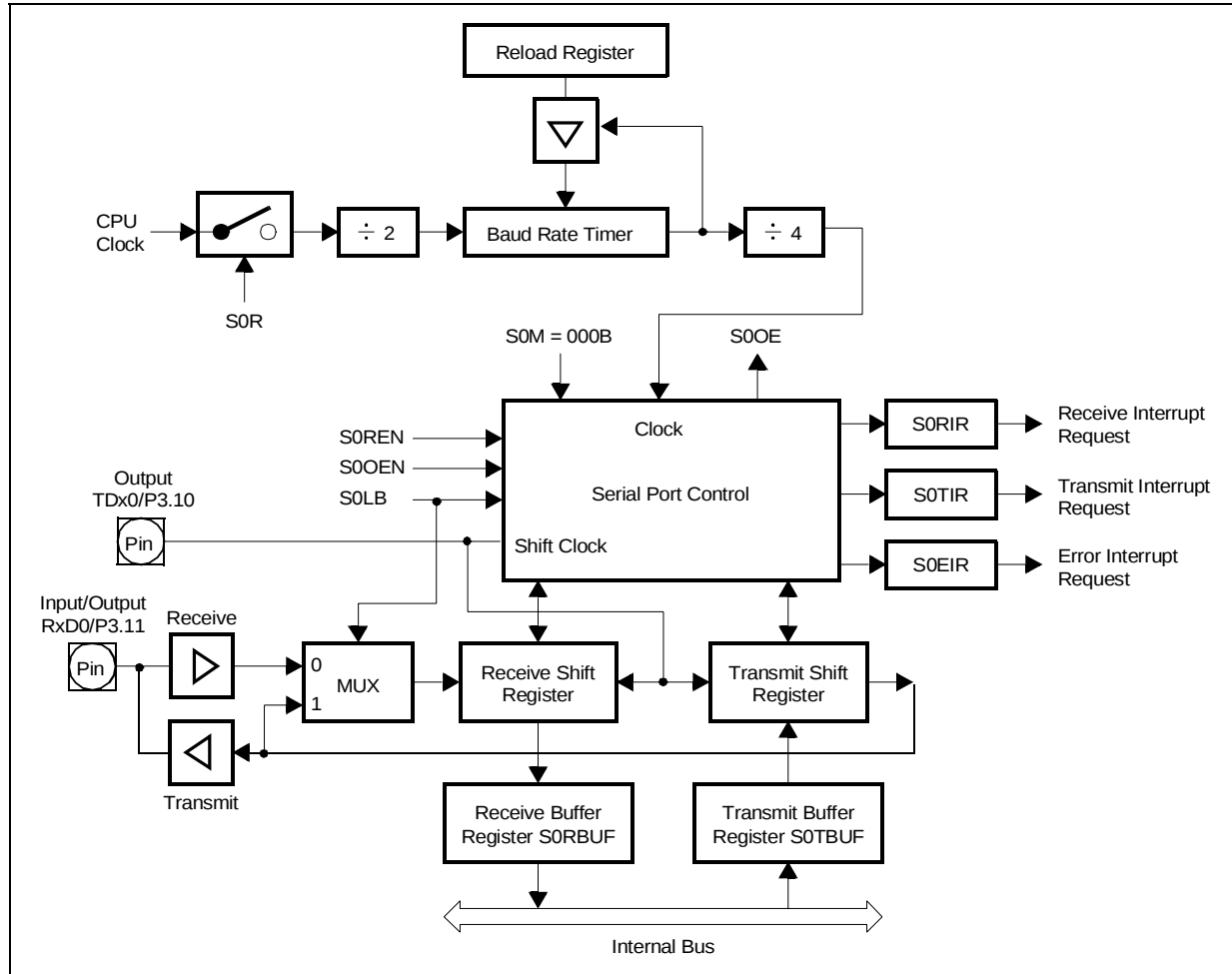
Figure 57 : Synchronous Mode of Serial Channel ASCO
