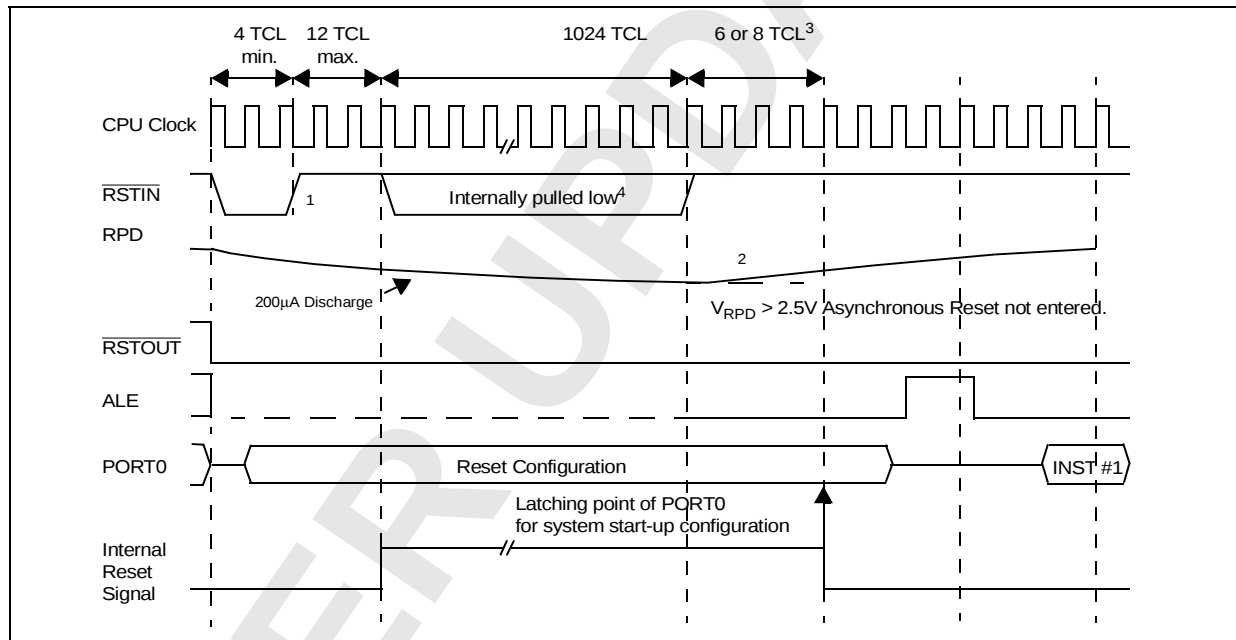
Figure 66 : Synchronous Warm Reset (Short low pulse on \overline{\text{RSTIN}} )
