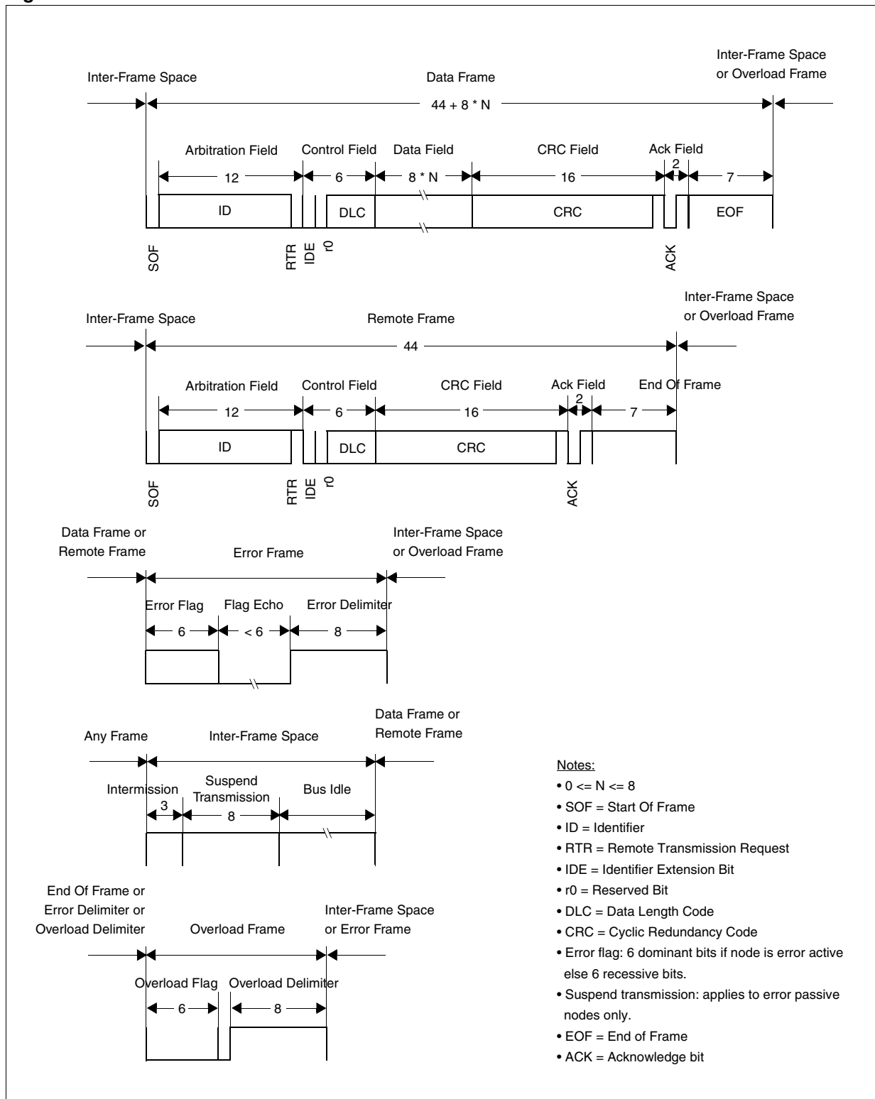
Figure 71. CAN frames
