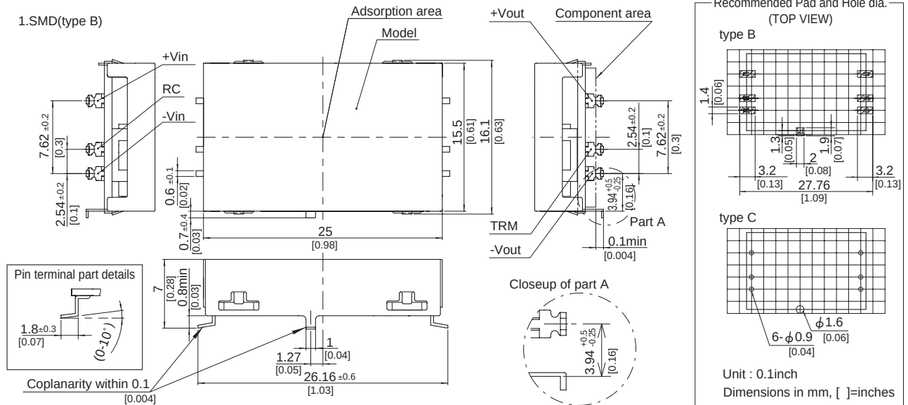
2.DIP(type C)
