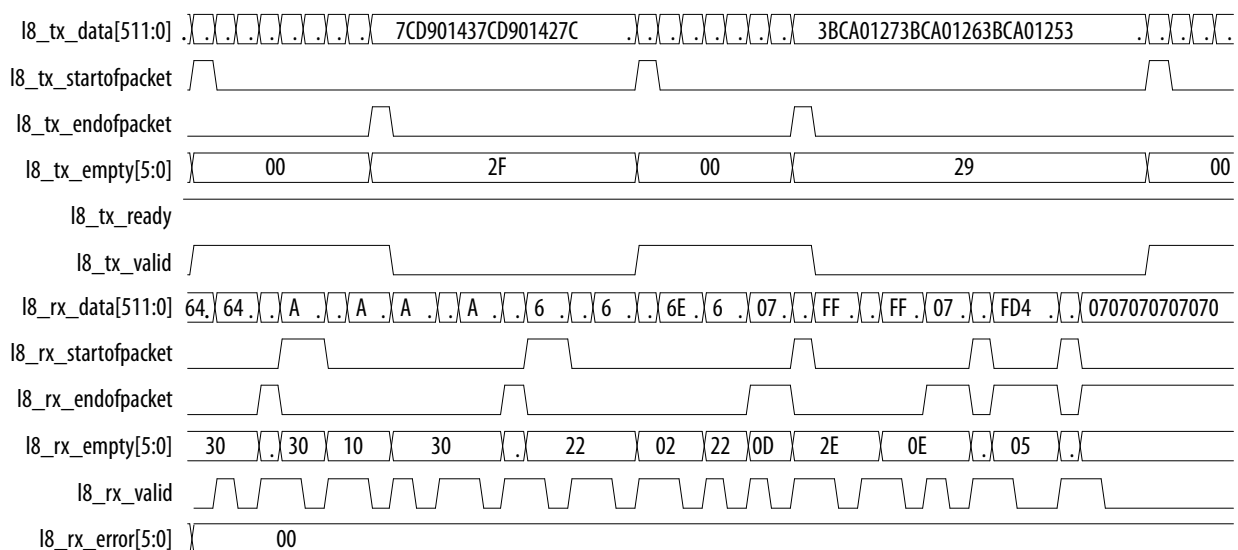
Figure 3-5: Traffic on the TX and RX Avalon-ST Client Interface for Low Latency 100GbE IP Core
