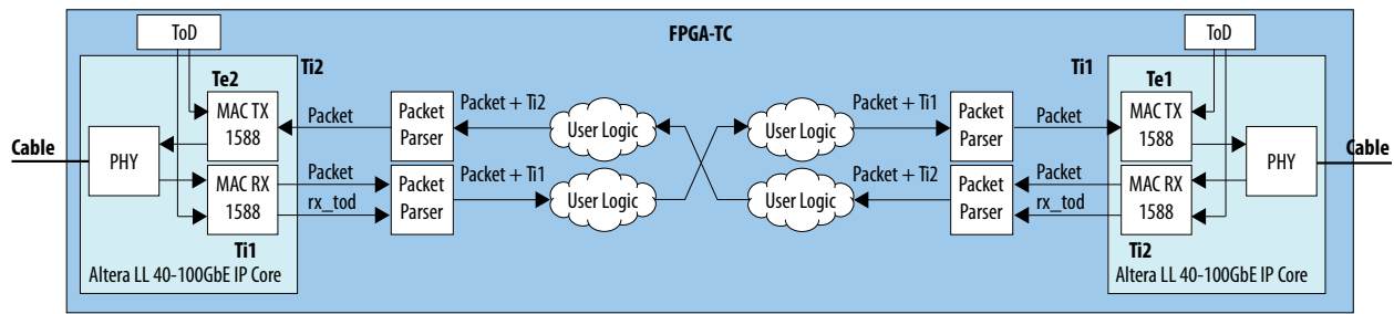
Figure 3-22: Software Flow Using Transparent Clock Mode System
