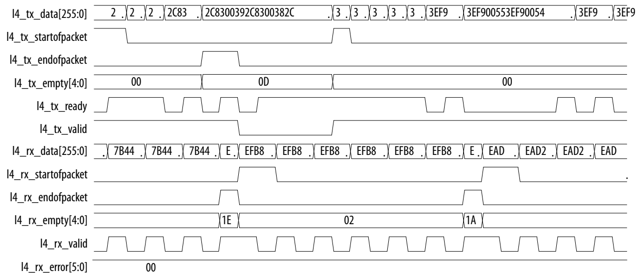
Figure 3-5: Traffic on the TX and RX Avalon-ST Client Interface for Low Latency 100GbE IP Core
