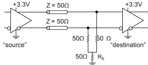
Figure 2. Three-Resistor ‘Y-Termination’
