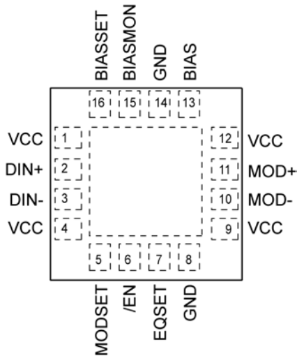
16-Pin QFN
